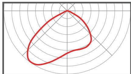
B4 - Asymmetric
