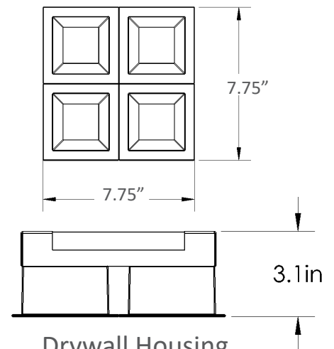
Drywall Housing
