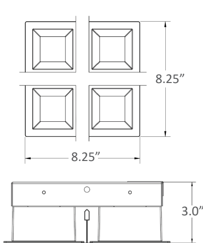
Flat Housing
