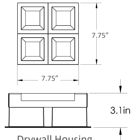
Drywall Housing
