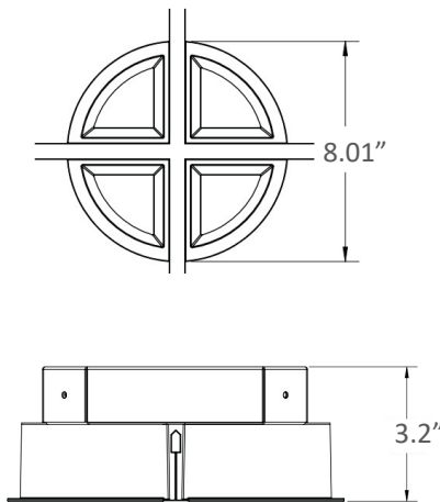
Flat Housing
