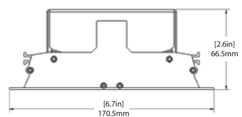
Height Dimensions
